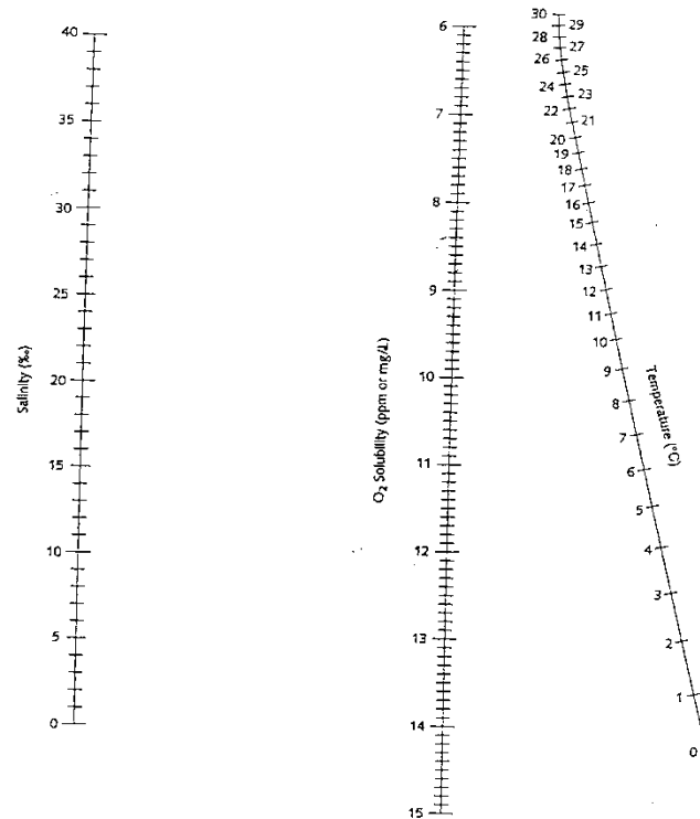
Figure 1.6 Nomograph of oxygen solubility in seawater. A straight line constructed between any two variables will intersect the third scale at the appropriate value of the third variable. Oxygen solubility in ppt (mL/L) can be obtained by multiplying mg/L by 0.7.
